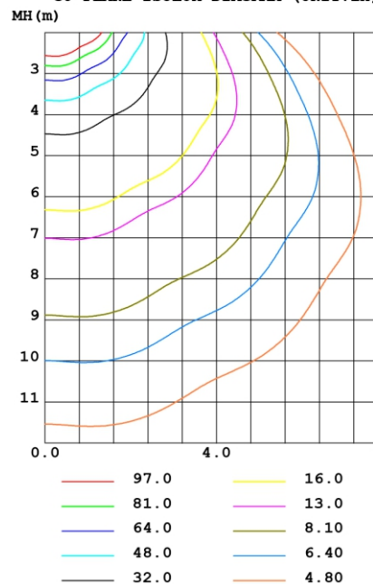
C0 PLANE ISOLUX DIAGRAM (UNIT:lx)
